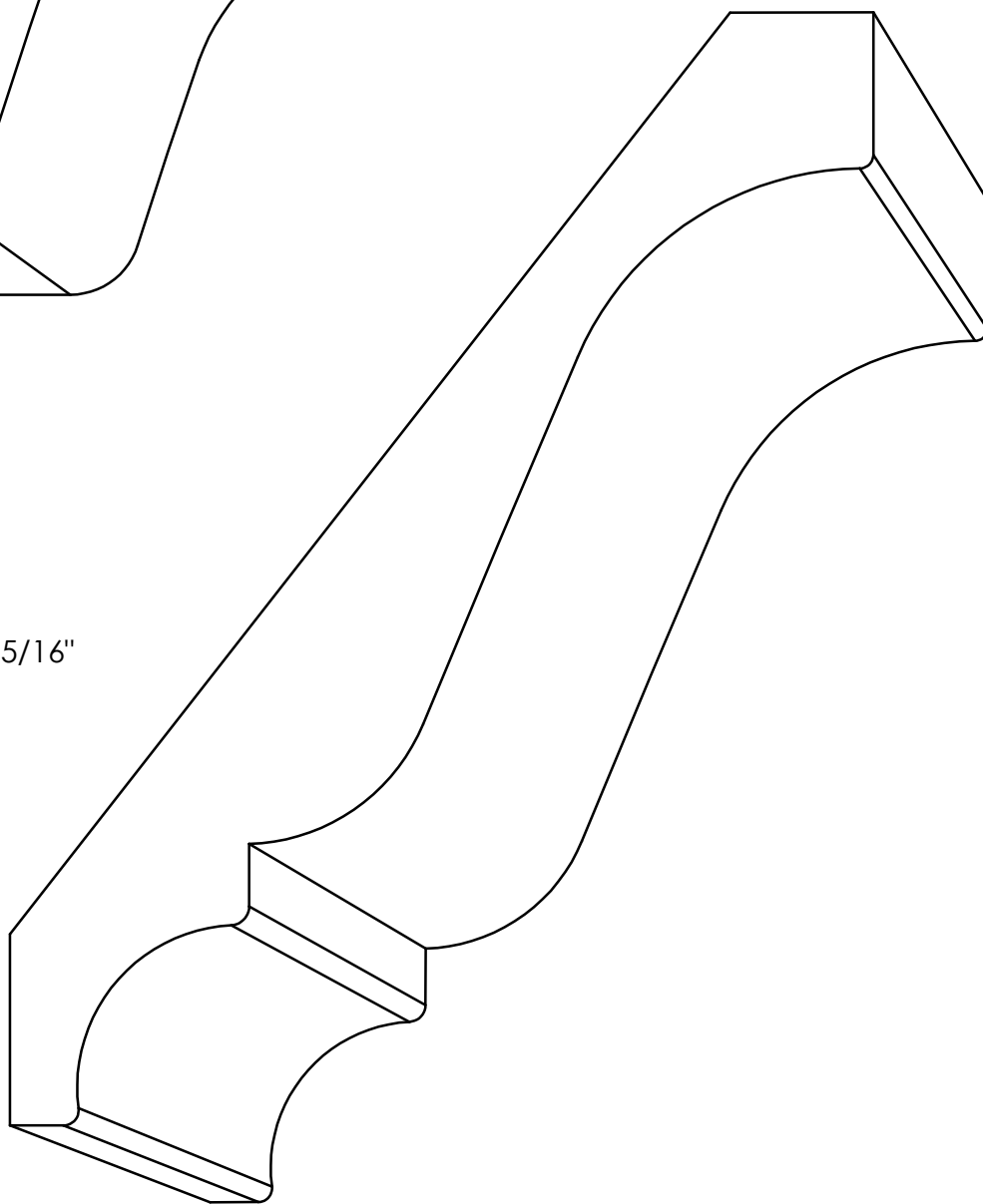
CR6 - 1-1/16" X 7-3/8" P= 4-1/2" - D=5-13/16"
