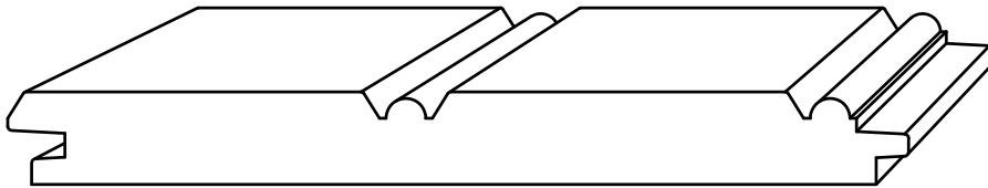
PL 4-4W - 7/16" x 4-1/4"
