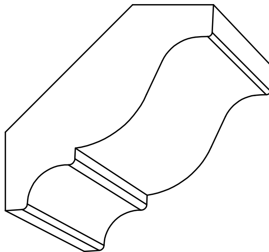
CR-259 - 13/16'' \times 3'' P= 2-1/8'' = D= 2-1/8''
