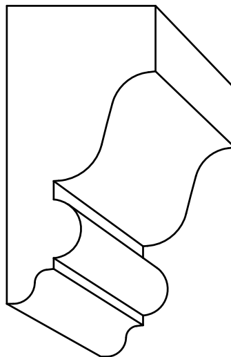
CR 2245 - 1\frac{1}{8} " x 2\frac{1}{4} " P= 1\frac{1}{8} " - D= 2\frac{1}{4} "
