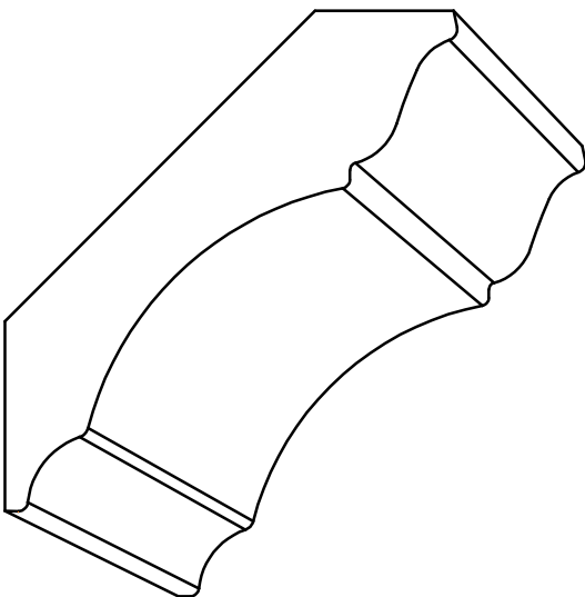
CR 68 - 11/16'' \times 3-5/32'' P= 2-3/32'' - D= 2-11/32''
