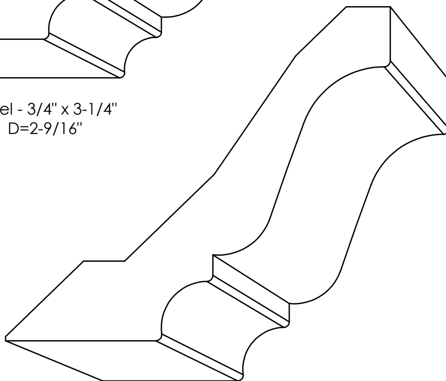
CR 4 w/ Heel - 3/4" \times 4-1/4" P= 2-21/32" - D= 3-13/32"
