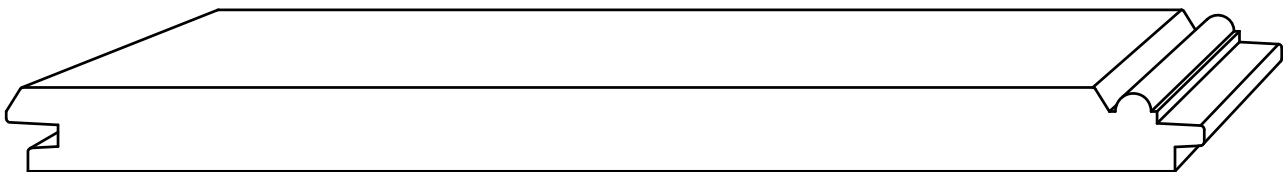
PL 3-6W - 7/16" x 6-1/4"
