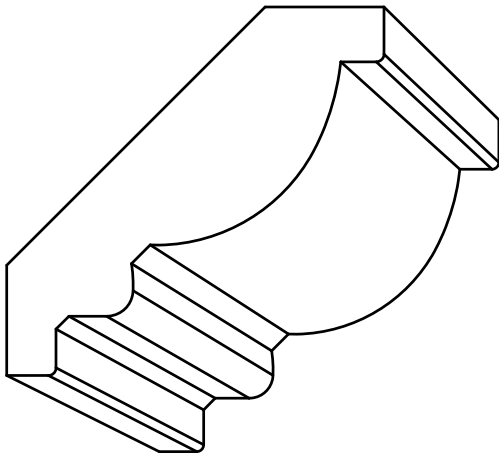
CR 31 - 3/4" x 2 - 3/4" P= 1 - 31/32" - D= 1 - 15/16"
