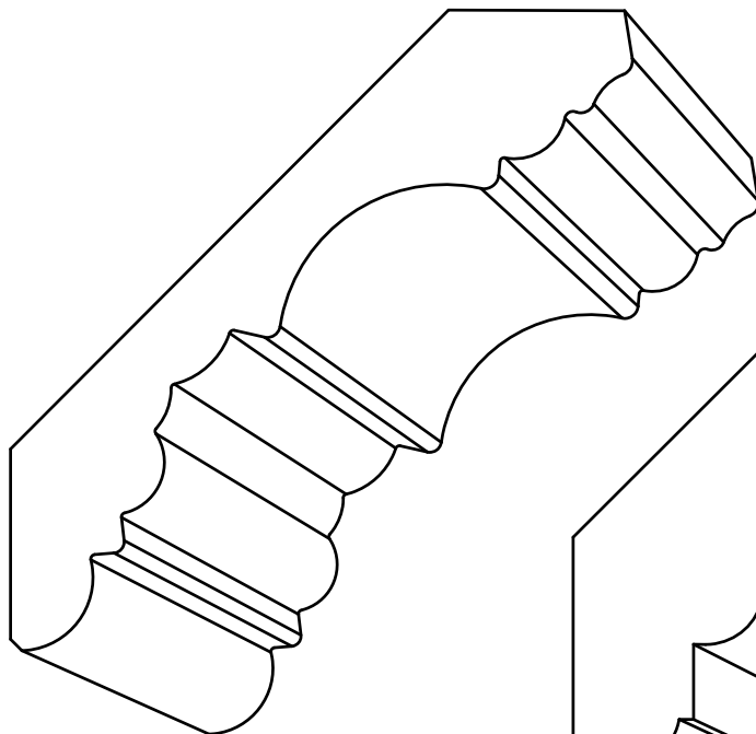
CR 4187 - 13/16" x 4-1/16" P= 2-15/16" - D= 3-1/16"
