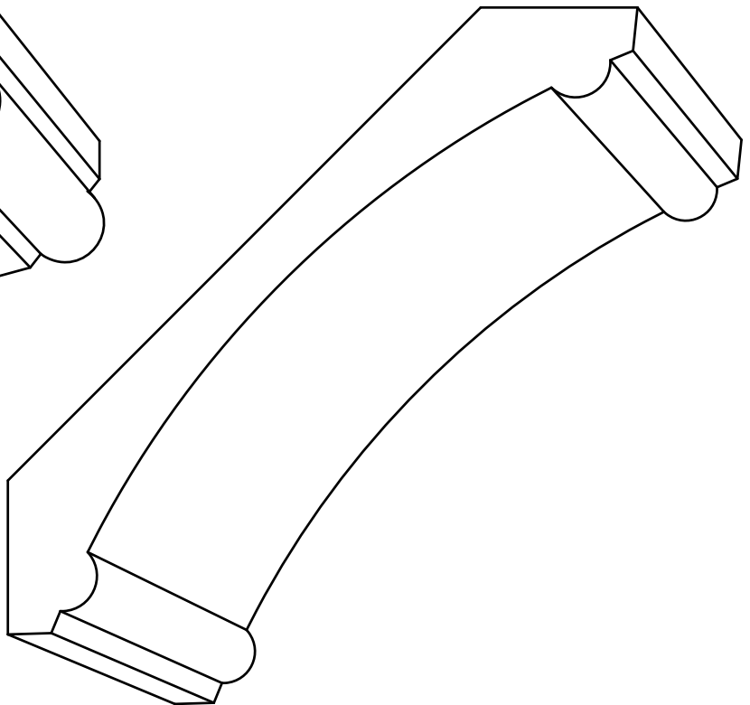
CR 3351 - 13/16" x 5-1/8" P= 3-5/8" - D= 3-5/8"
