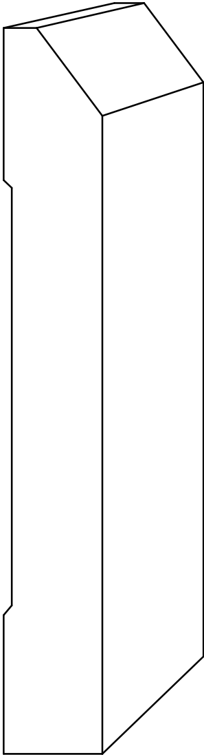
B 312 3/4" x 5-1/2" **
