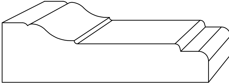
C 4794 PLYNTH - 1-1-16" x 3-21/32"
