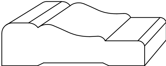
C 110 - 3/4" x 2-1/2"
