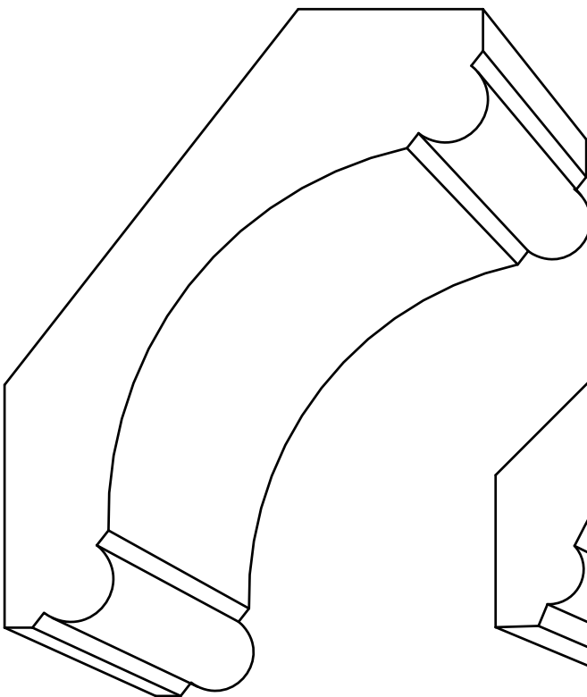
CR 3317 - 1-1/4" x 4-9/16" P= 2-25/32" - D= 3-19/32"
