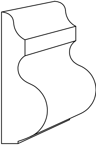
BC 183 13/16" x 2-11/32"
