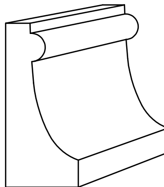
BC 187 3/4" x 1-11/16"
