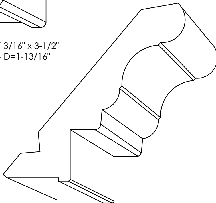
CR 4560 - 1" x 4\frac{7}{16} " P= 2\frac{3}{16} " - D= 3\frac{1}{4} "
