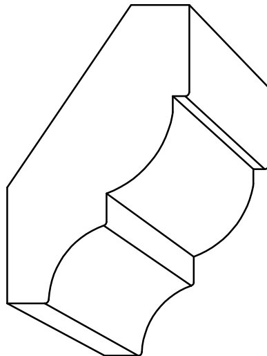
CR 2634 - \frac{3}{4}'' \times 2\frac{5}{8}'' P= 2\frac{1}{4}'' - D= 1\frac{3}{8}''
