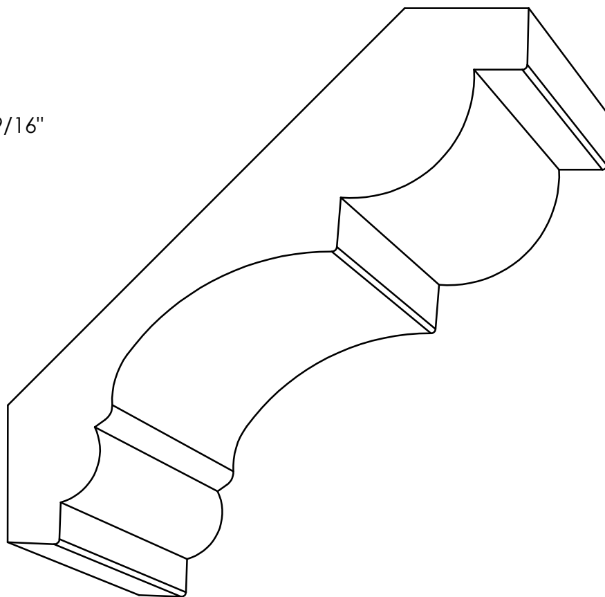
CR 5058 - 1'' \times 5-9/16'' P= 3-15/16'' - D= 4-1/32''
