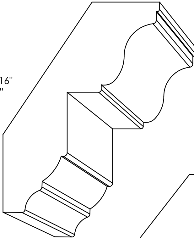
CR 4342 - 1\frac{1}{16} " x 4\frac{11}{32} " P= 2\frac{19}{32} " - D= 3\frac{1}{2} "
