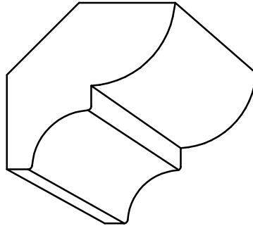
CR 10 - 5/8" \times 1-3/4" P= 1-1/4" - D= 1-7/32"
