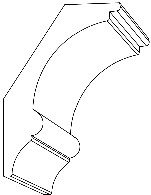
CR 4345 - 1'' \times 4-11/32'' P= 2-7/16'' - D= 3-5/8''
