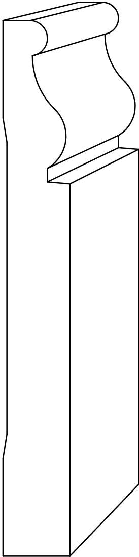
B 40 1 1/16" x 5-1/2" **
