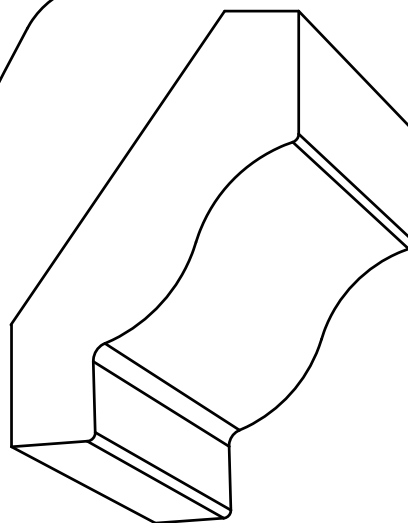
CR 2720 - 11/16" x 2-23/32" P= 1-1/2" - D= 2-1/4"
