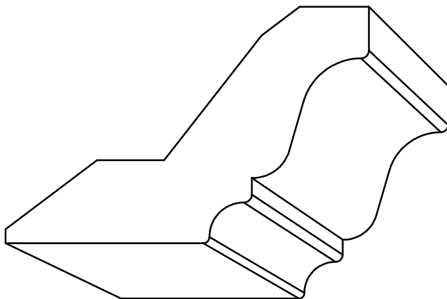
CR 2 w/ Heel - 5/8" \times 2-1/4" P= 1-17/32" - D= 1-25/32"
