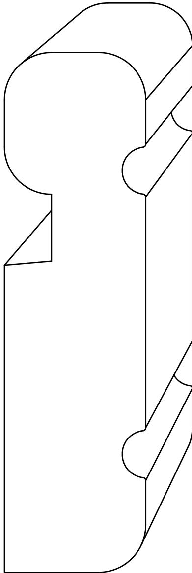
HR 1500 - 1-1/2" x 5-1/2"
