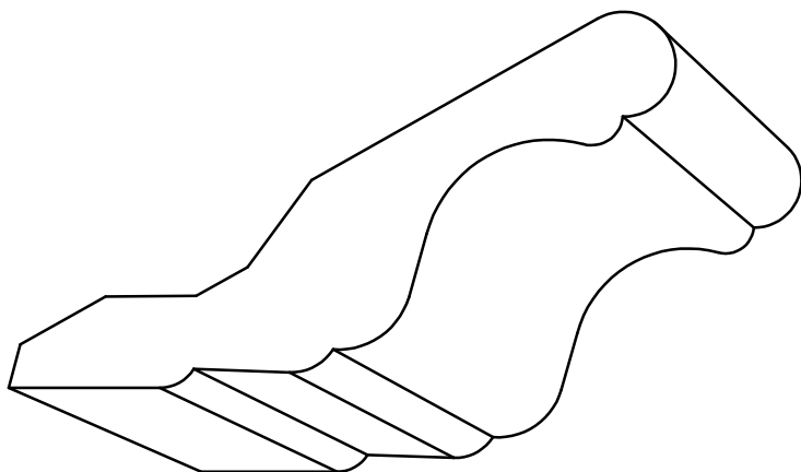
CR 4540 - 1\frac{13}{16} " x 3\frac{9}{16} " P= 2\frac{15}{32} " - D= 1\frac{25}{32} "
