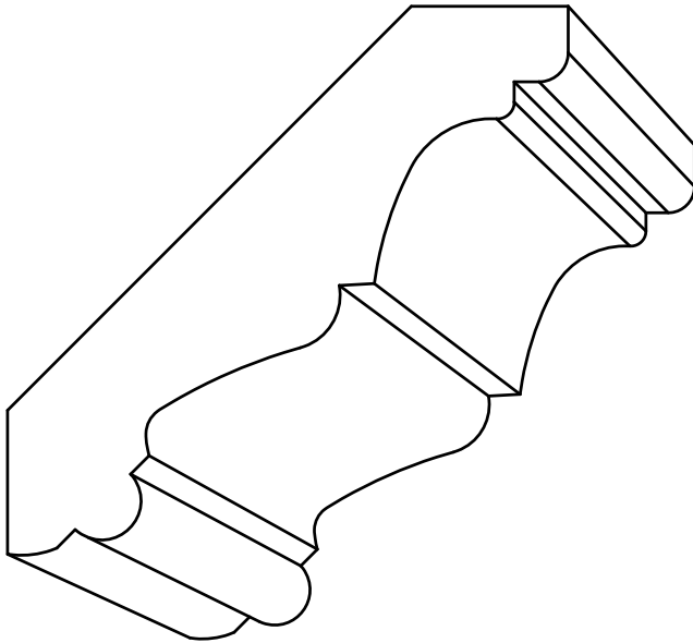
CR 3750 - 13/16" x 3-3/4" P= 2-11/16" - D= 2-5/8"
