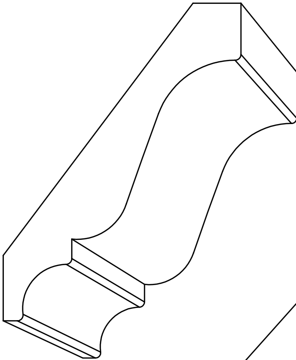
CR 4 - \frac{3}{4} " x 4\frac{1}{4} " P= 2\frac{17}{32} " - D= 3\frac{13}{32} "
