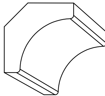
CV 134 - \frac{3}{4} " x 1\frac{3}{4} " P= 1\frac{1}{4} " - D= 1\frac{1}{4} "
