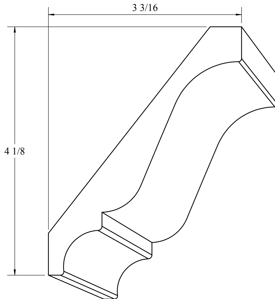
CR 5 - \frac{3}{4} " x 5\frac{1}{4} " P= 3\frac{3}{16} " - D= 4\frac{1}{8} "
