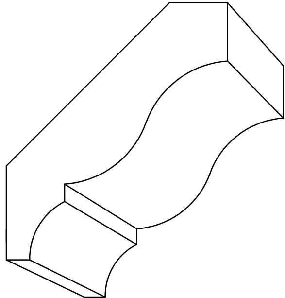
CR 3629 - 13/16" x 3-5/8" P= 2-3/8" - D= 2-3/4"
