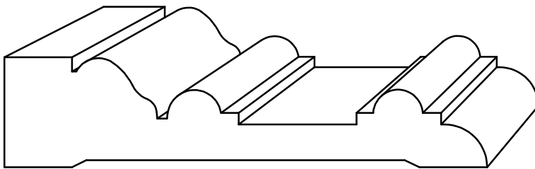
C 2876 - 13/16" x 3-9/16"
