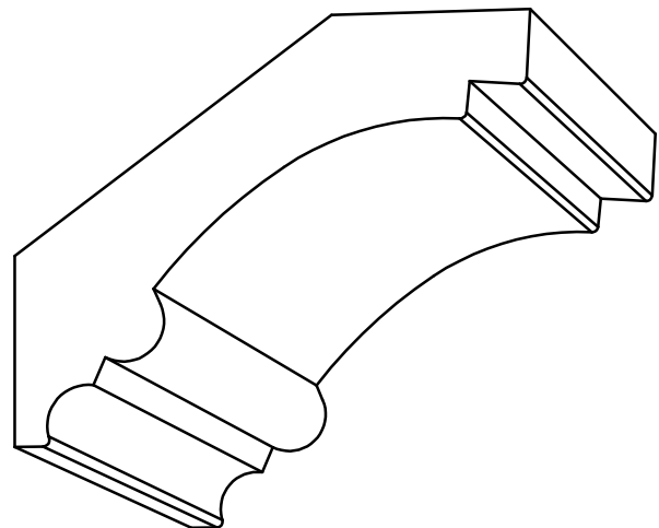
CR 3073 - 1\frac{13}{16} " x 3\frac{7}{32} " P= 2\frac{15}{32} " - D= 2\frac{3}{32} "
