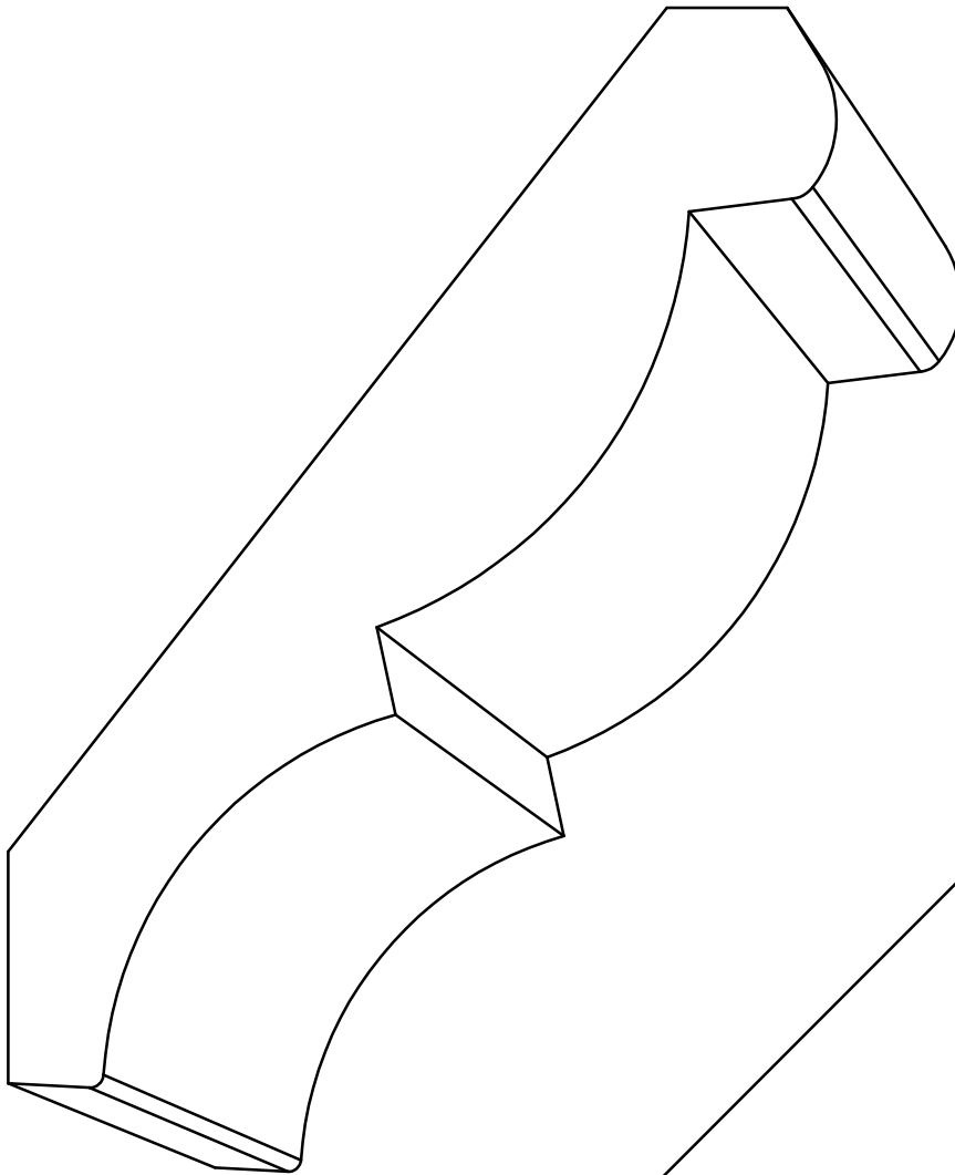
CR 92 - 1\frac{1}{16}'' \times 6\frac{1}{4}'' P= 3\frac{29}{32}'' - D= 5\frac{3}{32}''
