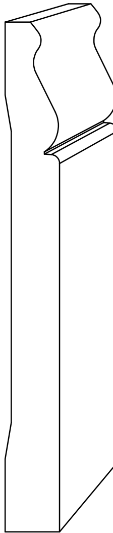
B 59 9/16" x 5-1/4" **
