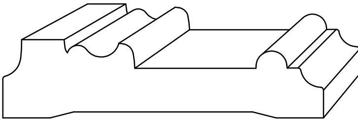
C 3390 - 13/16" x 3-3/8"
