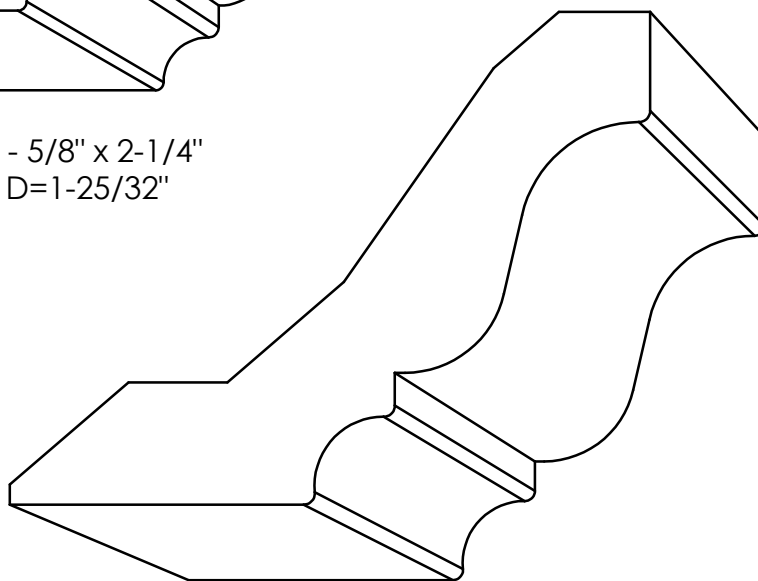
CR 3 w/ Heel - 3/4" \times 3-1/4" P= 2-5/32" - D= 2-9/16"
