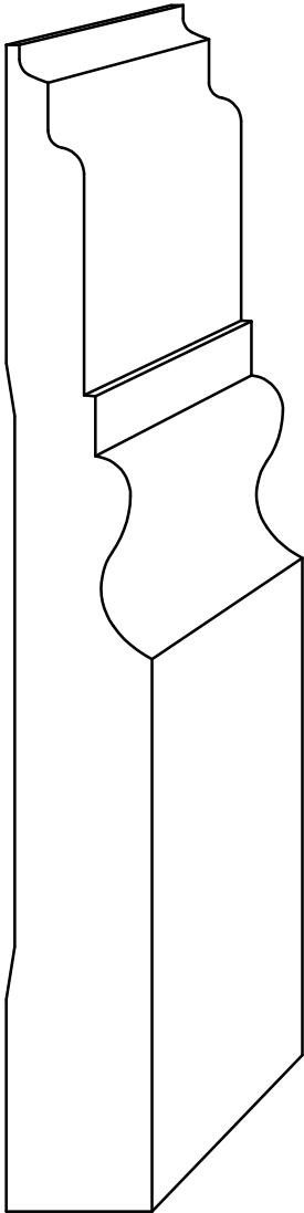
B 49 11/16" x 5-1/2" **
