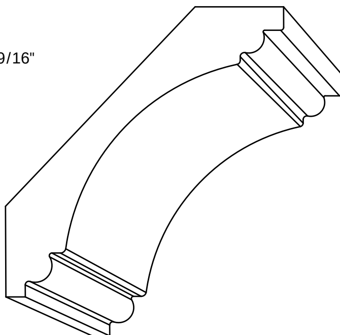
CR 3325 - \frac{13}{16} " x 4\frac{1}{8} " P= 2\frac{7}{8} " - D= 2\frac{7}{8} "
