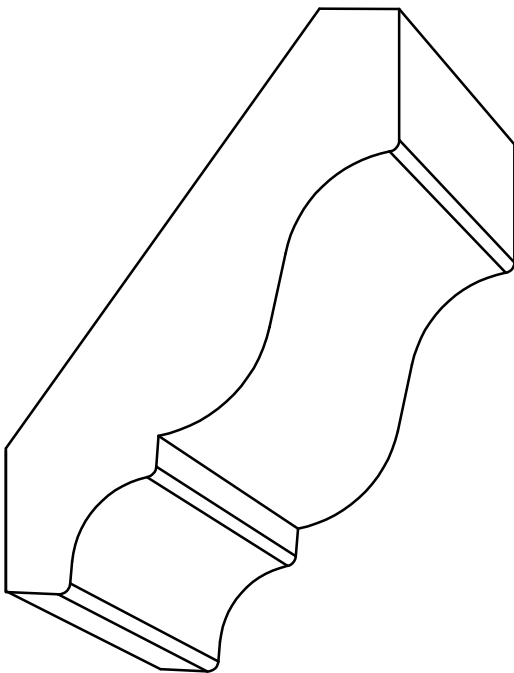
CR 3665 - 13/16" x 3-21/32" P= 2-1/16" - D= 3-1/16"
