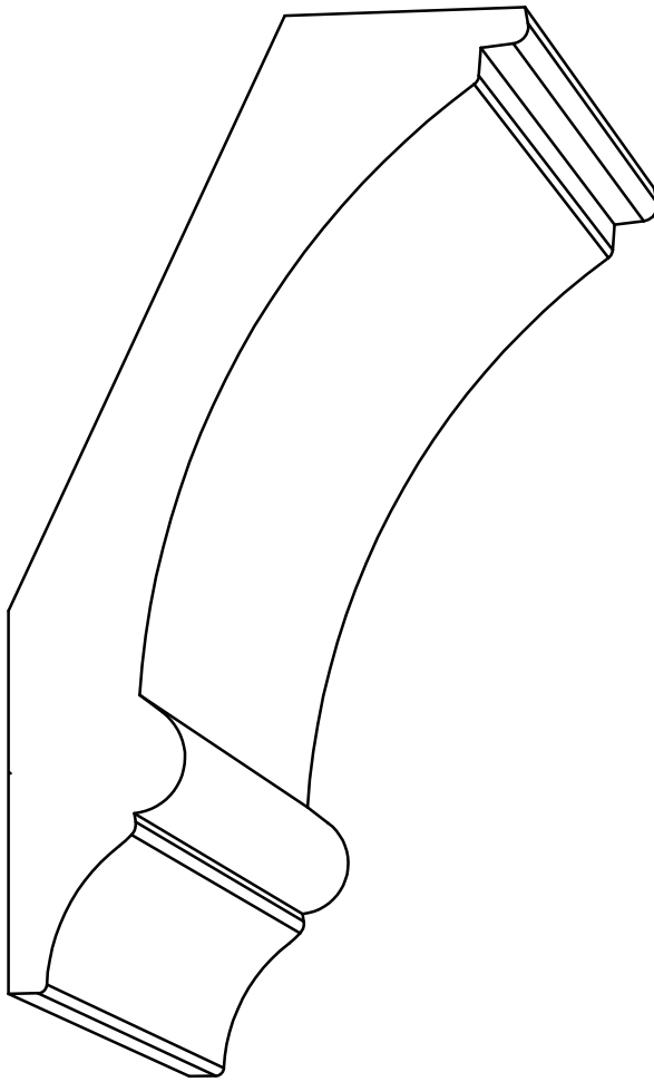
CR 4355 - 1\frac{1}{16}'' \times 5\frac{7}{32}'' P= 2\frac{7}{16}'' - D= 4\frac{5}{8}''
