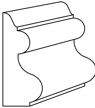
BC 172 11/16" x 1-5/8"
