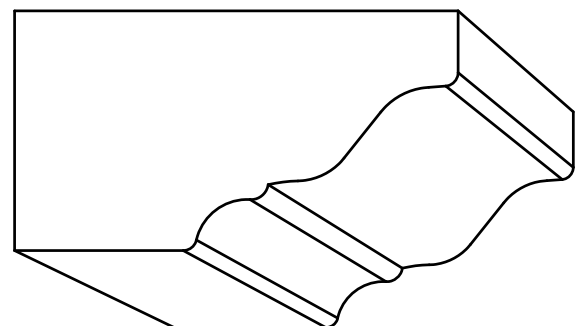
CR 24TM - 1-1/4" x 2-5/16" P= 2-5/16" - D= 1-1/4"
