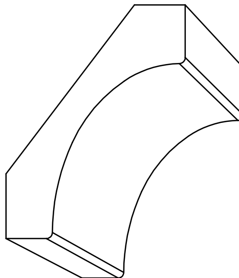
CV 300 - 3/4" x 3" P= 1-13/16" - D= 2-3/8"
