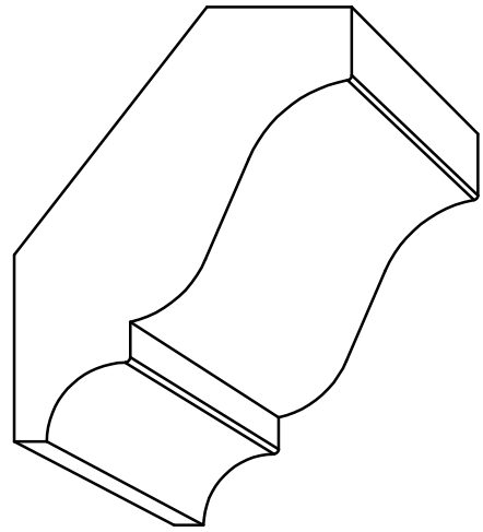
CR 258 - 3/4'' \times 2-5/8'' P= 1-5/8'' - D= 2-1/16''
