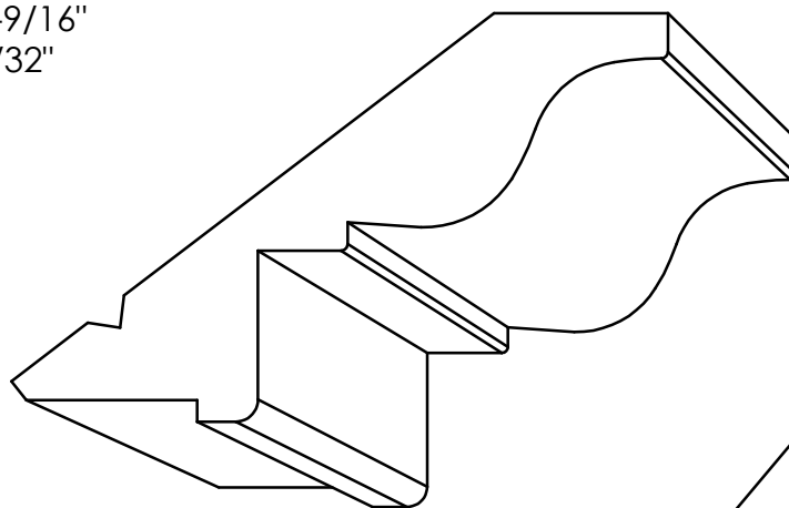
CR 4550 - 1\frac{13}{16} " x 3\frac{1}{2} " P= 2\frac{7}{32} " - D= 1\frac{13}{16} "
