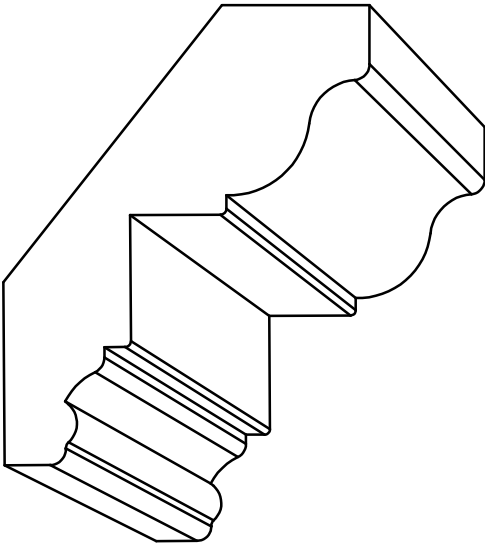
CR 3340 - 1\frac{13}{16} " x 3\frac{1}{16} " P= 1\frac{29}{32} " - D= 2\frac{13}{32} "
