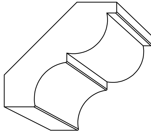
CR 2058 - \frac{3}{4}'' \times 2\frac{5}{8}'' P= 1\frac{15}{16}'' - D= 1\frac{25}{32}''
