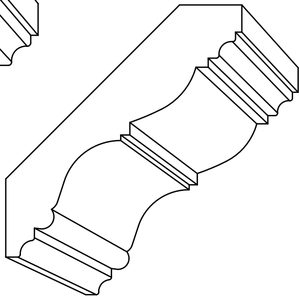
CR 4024 - 11/16" x 3 - 11/16" P= 2 - 17/32" - D= 2 - 11/16"
