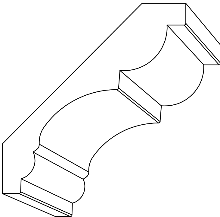
CR 4058 - 13/16'' \times 4-9/16'' P= 3-3/16'' - D= 3-9/32''
