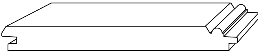
PL 3-4W - 7/16" x 4-1/4"
