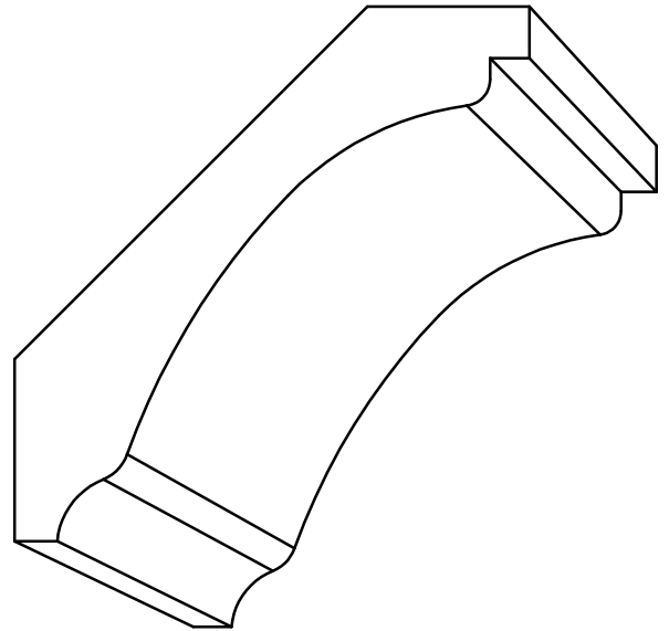
CR 3074 - 3/4'' \times 3-1/2'' P= 2-7/16'' - D= 2-17/32''
