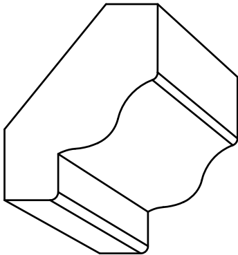
CR 2370 - 5/8" x 1-7/8" P= 1-3/16" - D= 1-15/32"
