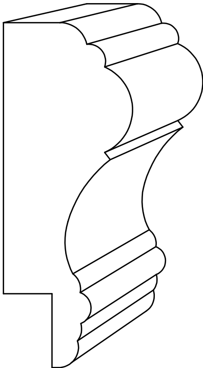
CHR 312 - 1-5/16" x 3-1/2"
