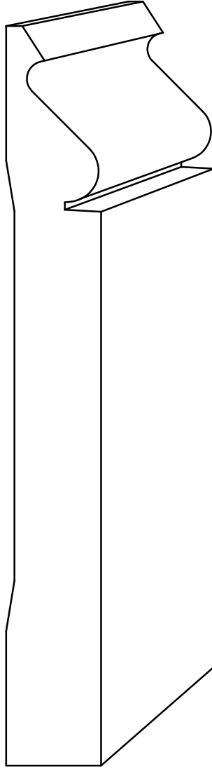
B 163 1 1/16" x 5-1/2" **
