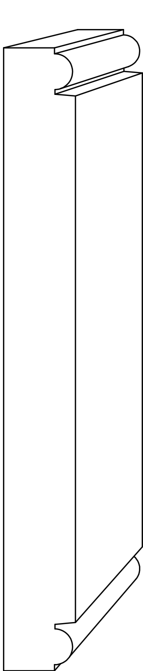
CHR 280 - 3/4" x 6-1/2"
