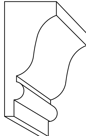
CR 2275 - 1\frac{1}{32} " x 2\frac{9}{32} " P= 1\frac{1}{32} " - D= 2\frac{9}{32} "
