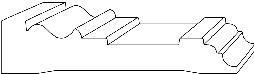
C 4795 - 1-3/32" x 4-25/32"
