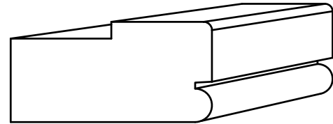
LR 105 - 3/4" x 1-1/2"
