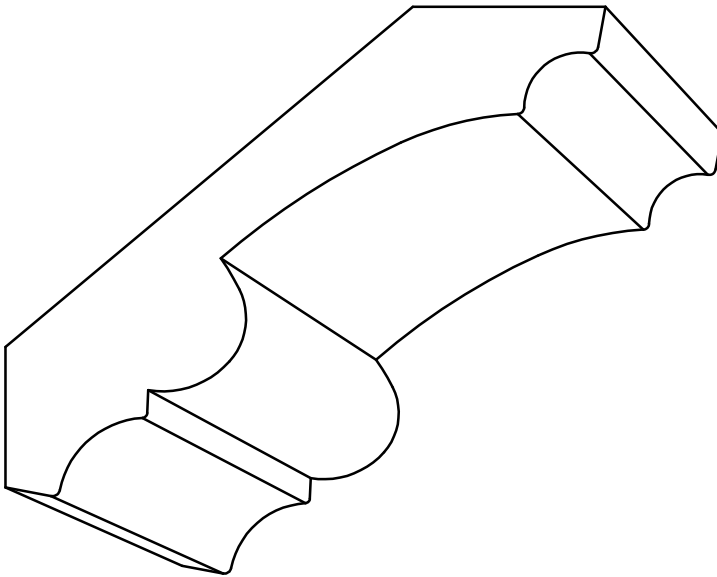
CR 3078 - 1\frac{13}{16} " x 4" P= 3\frac{1}{8} " - D= 2\frac{1}{2} "
