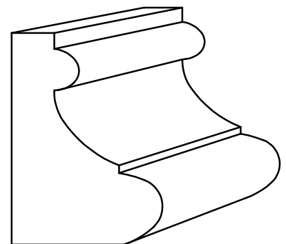
BC 600 1-1/8" x 1-19/32"
