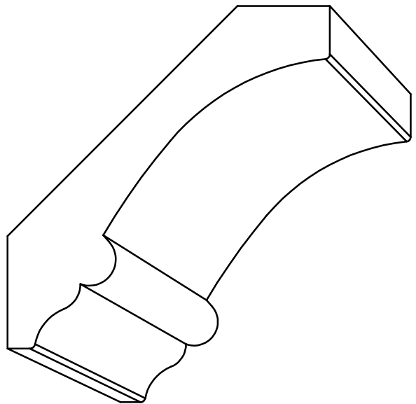
CR 3075 - 3/4'' \times 3-1/2'' P= 2-11/32'' - D= 2-19/32''
