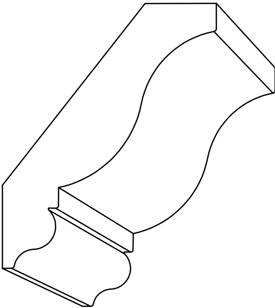
CR 3640 - \frac{3}{4} " x 3\frac{17}{32} " P= 2\frac{1}{4} " - D= 2\frac{3}{4} "
