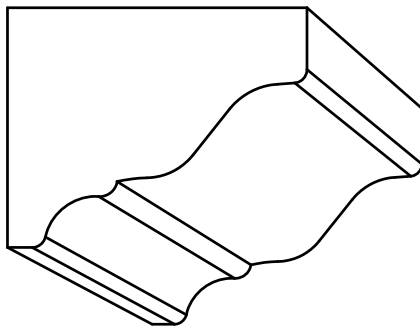
CR 24 - 1-1/4" x 1-9/16" P=1-9/16" - D=1-1/4"
