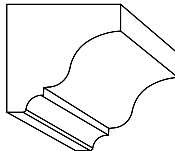
CR 15 - 1-1/8" x 1-3/16" P=1-3/16" - D=1-1/8"
