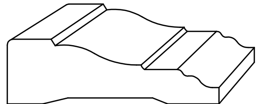
C 108 - 11/16" x 2-1/4"
