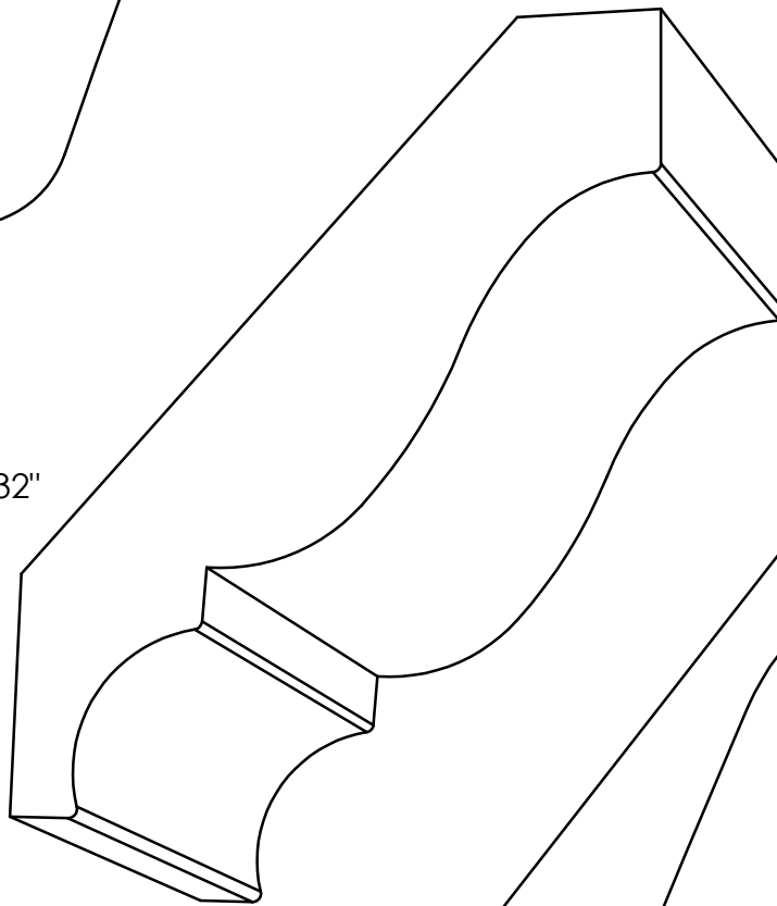
CR4968 - 1" X 4\frac{31}{32} " P= 3\frac{1}{8} " - D= 3\frac{7}{8} "
